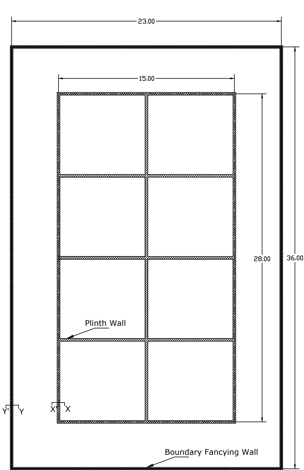
plinth wall Layout
